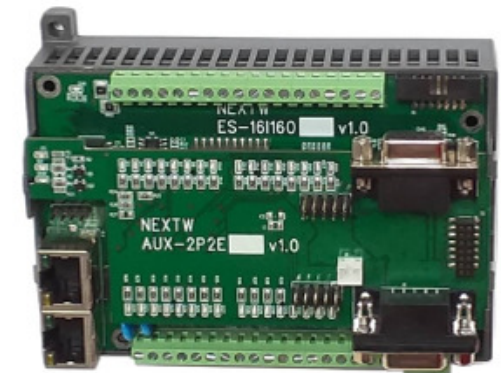
ES-16I16O & AUX-2P2E 16I/16O High Speed Pulse & Encoder Module
